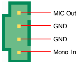
MODEM-CN
