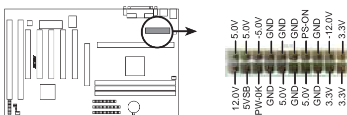
ATX Power Connector
