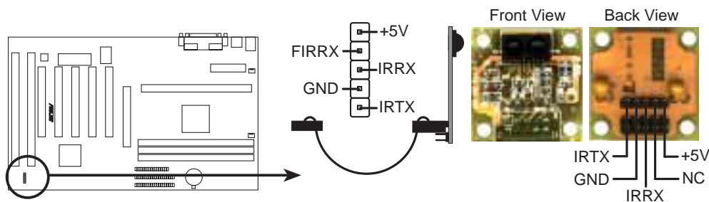
Infrared Module Connector
