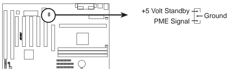
Wake on LAN Connector
