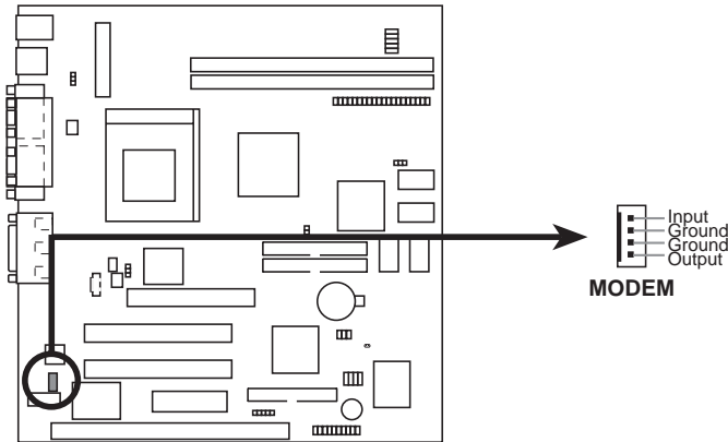
MEZ-VM Voice Modem In Connector
