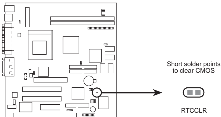
MEZ-VM Clear RTC RAM
