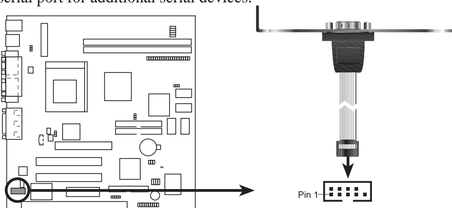
MEZ-VM Serial COM 2 Header
