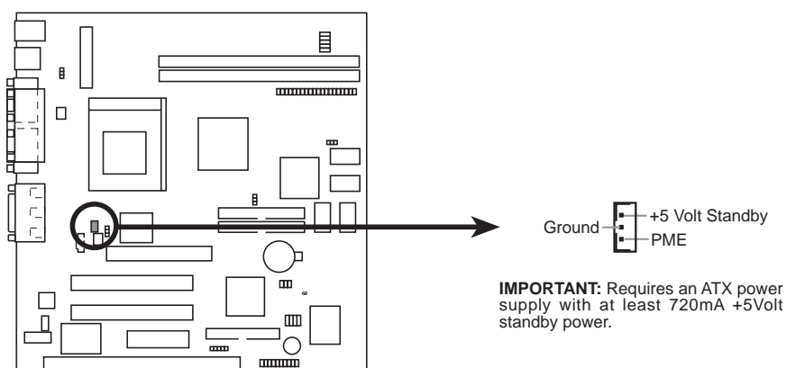
MEZ-VM Wake-On-LAN Connector
