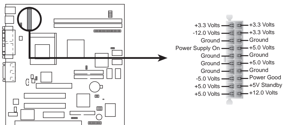
MEZ-VM ATX Power Connector
