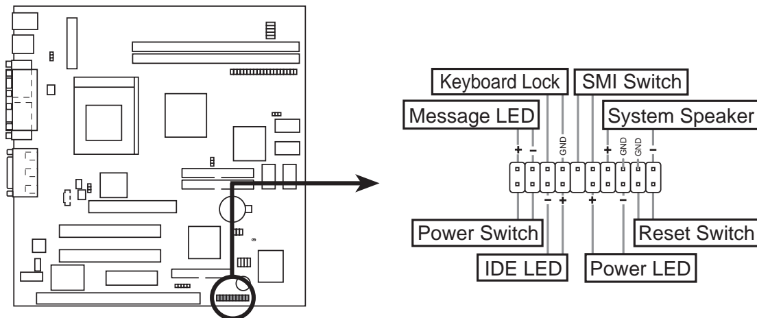
MEZ-VM System Panel Connectors
