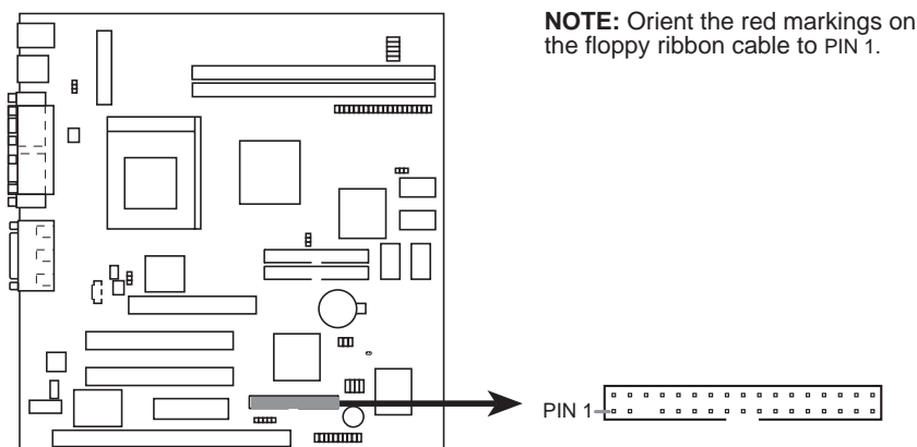
MEZ-VM Floppy Disk Drive Connector
