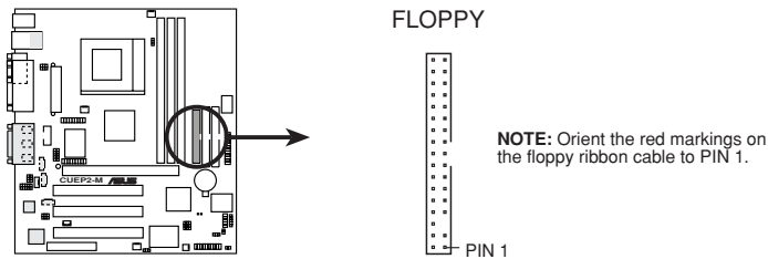
CUEP2-M Floppy Disk Drive Connector
