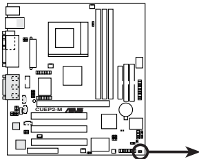
CUEP2-M IDE Activity LED
