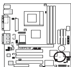
CUPE2-M Clear RTC RAM
