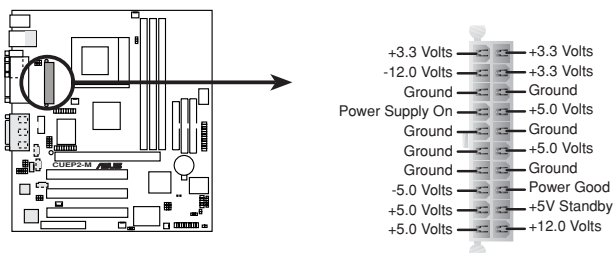
CUEP2-M ATX Power Connector
