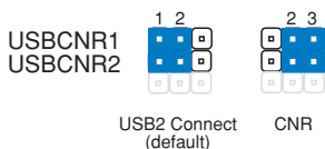
CUEP2-M USB/CNR Selection
