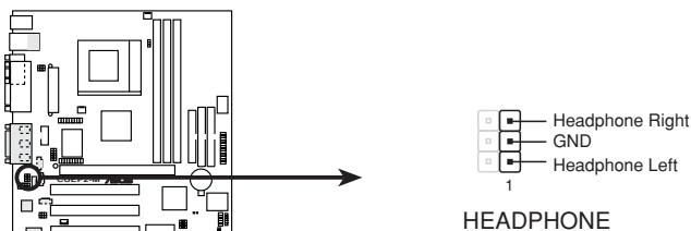
CUEP2-M True-Level Line Out Header
