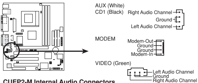
CUEP2-M Internal Audio Connectors
