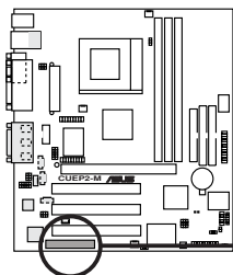
CUEP2-M Communication & Networking Riser Connectors
