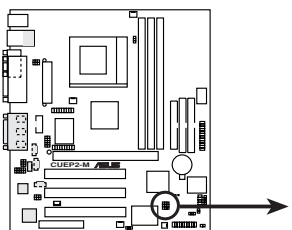
CUEP2-M USB/CNR Selection
