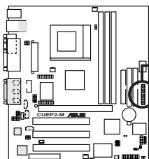
CUEP2-M Front Panel Connectors
