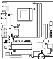
CUEP2-M Wake-On-Ring Connector
