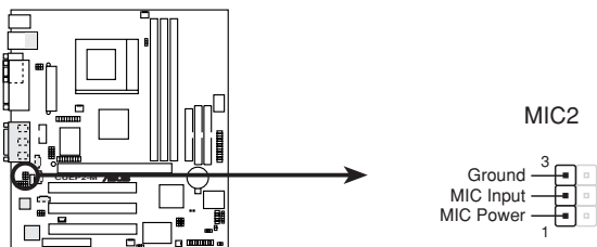
CUEP2-M Internal Microphone Connector
