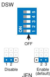
CUEP2-M JumperFree™ Mode Setting
