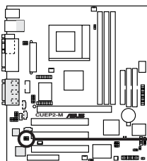
CUEP2-M On Board Lan Setting
