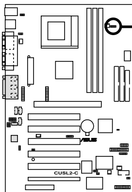
CUSL2-C VIO Setting
