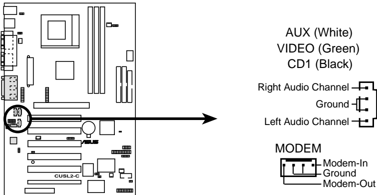
CUSL2-C Internal Audio Connectors
