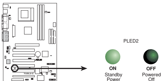
TUSL2-C Onboard LED
