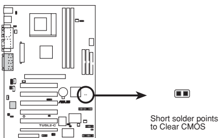
TUSL2-C Clear RTC RAM
