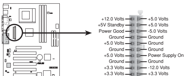
TUSL2-C ATX Power Connector
