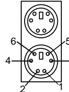
PS/2 Keyboard
