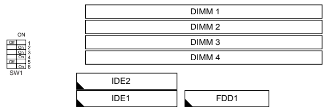
Figure 2–2. CPU Type Configuration
