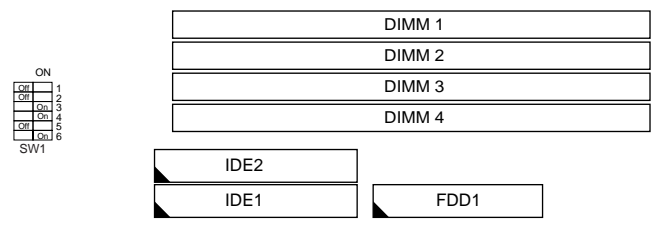
Figure 2–4. CPU Type Configuration
