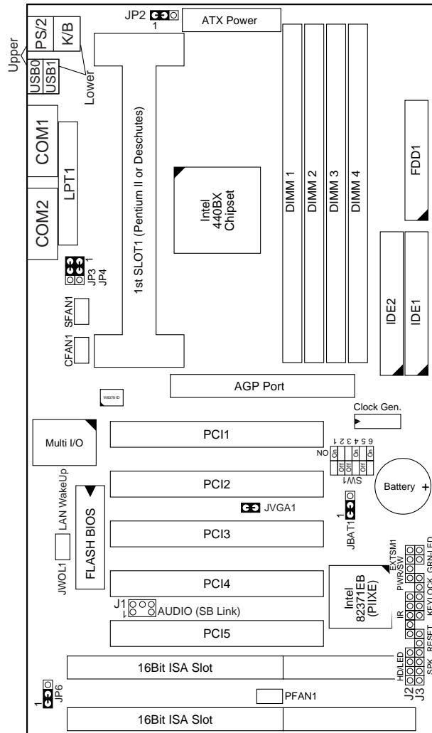
Figure 1-1. Motherboard Layout
