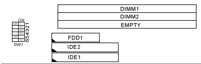
Figure 2-2 CPU Type Configuration
