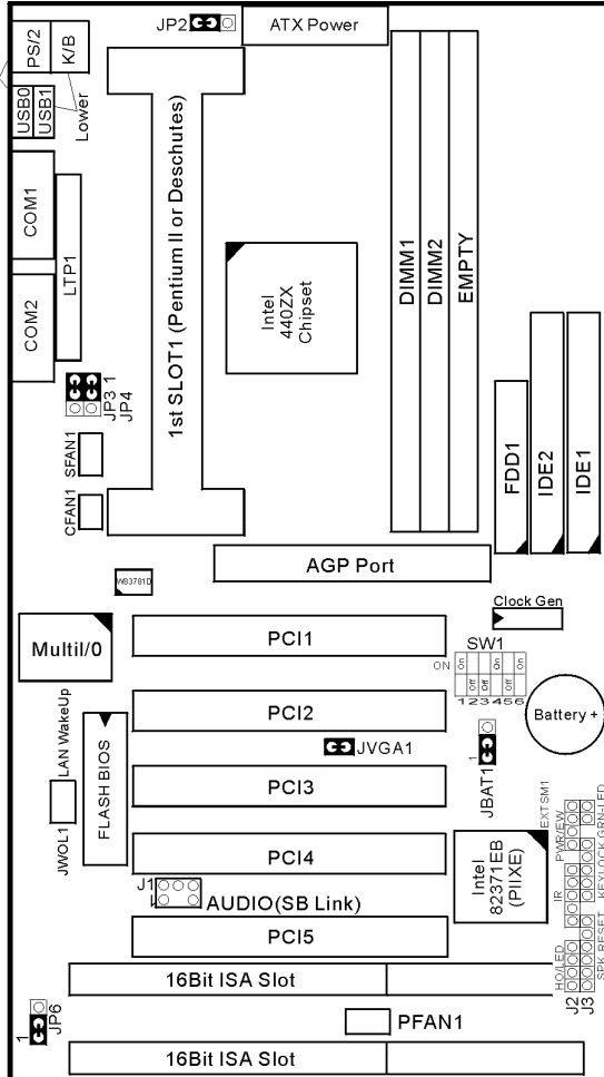
Figure 1-1. Motherboard Layout
