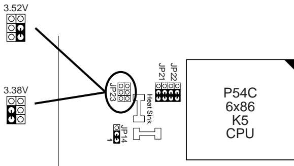
Figure 2-12-2. CPU Type Configuration
