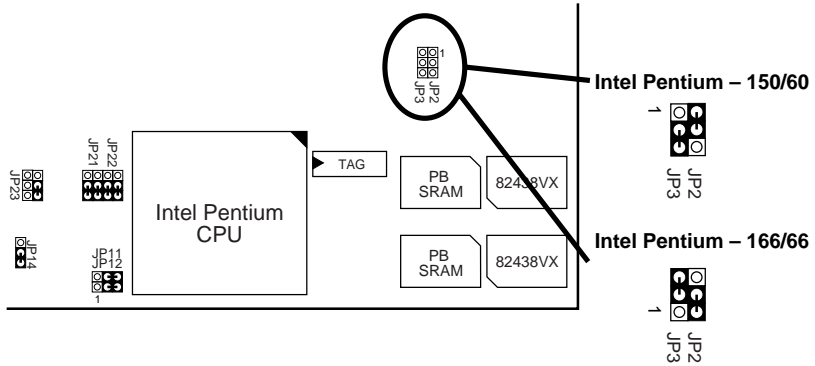
Figure 2-7. INTEL Pentium CPU Type Configuration
