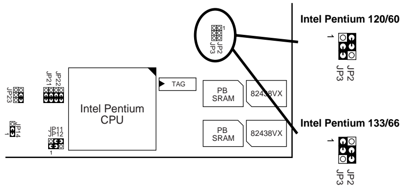
Figure 2-6. INTEL Pentium CPU Type Configuration
