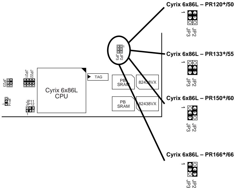
Figure 2–4. Cyrix 6x86L CPU Type Configuration
