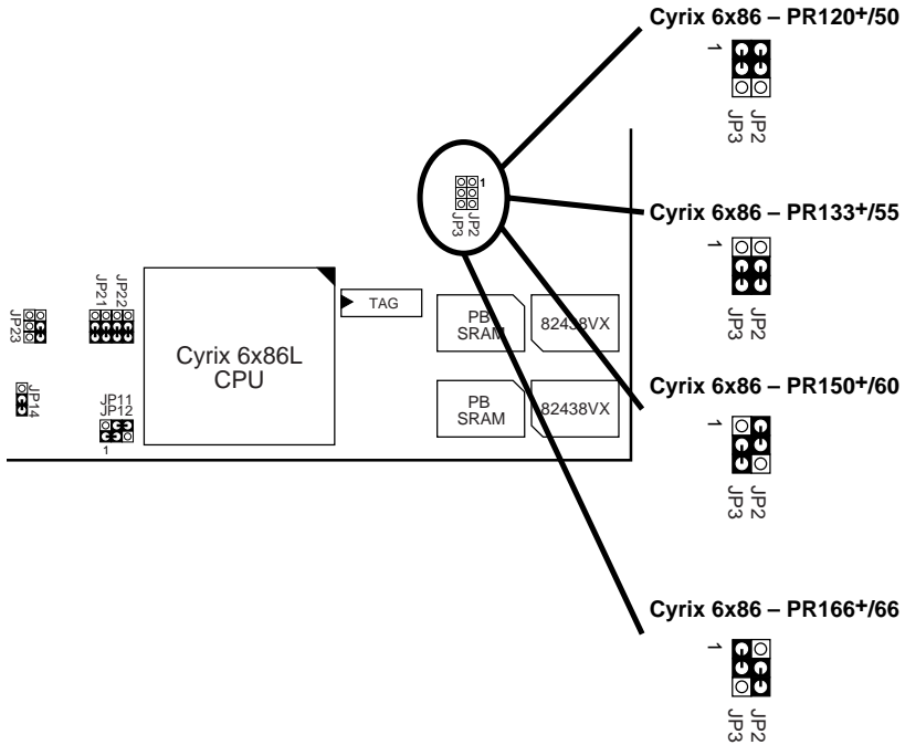
Figure 2–9. Cyrix 6x86 CPU Type Configuration
