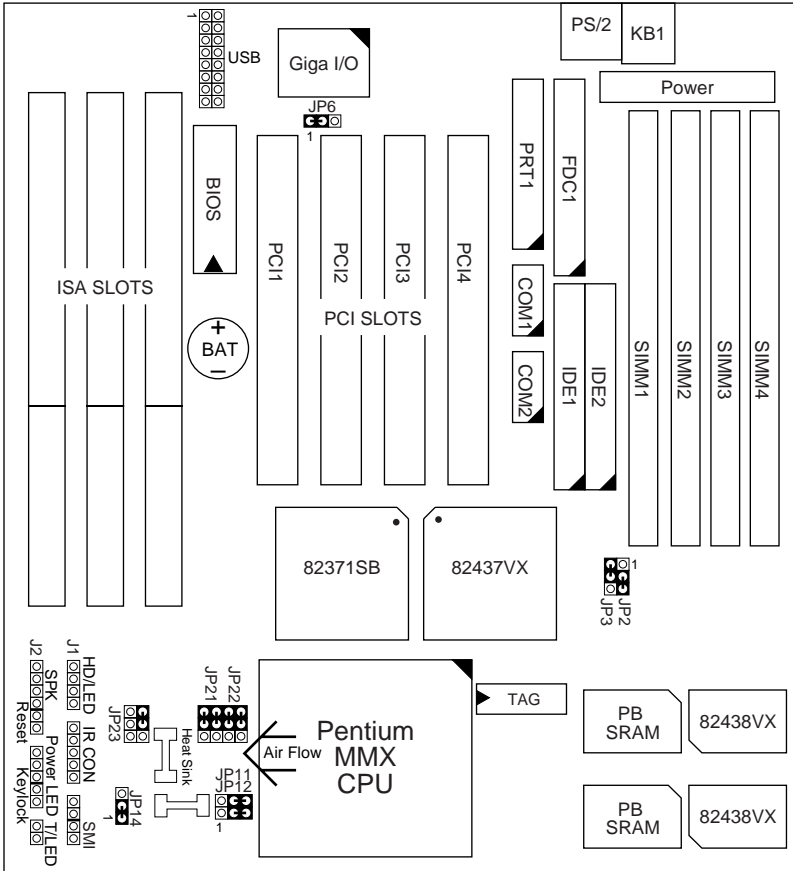
Figure 1-1. SL-53A2/A5 Motherboard Layout
