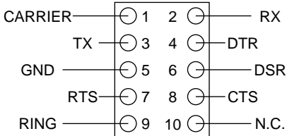
COM1/2 (Top View)
