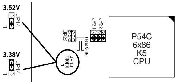
Figure 2-12-1. CPU Type Configuration
