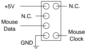
MS1 Top View
