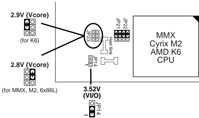
Figure 2-12-3 CPU Type Configuration
