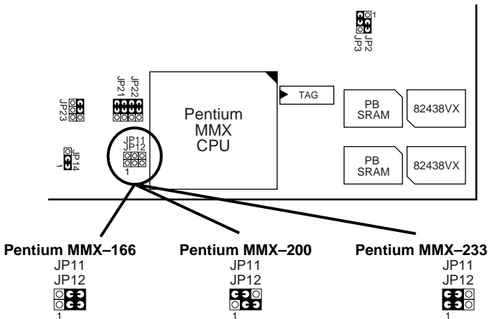
Figure 2-1. INTEL Pentium MMX CPU Type Configuration
