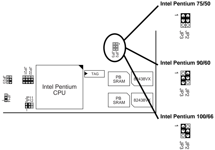
Figure 2-5. INTEL Pentium CPU Type Configuration
