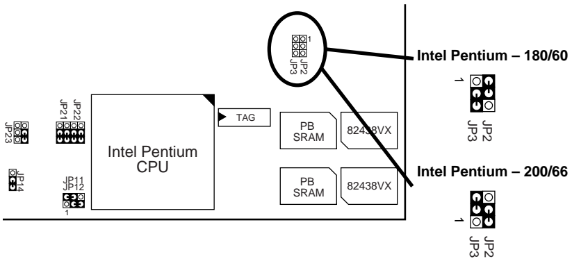
Figure 2-8. NTEL Pentium CPU Type Configuration
