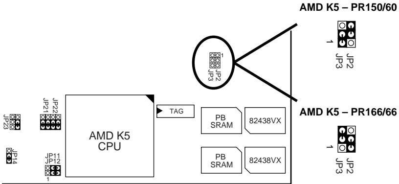
Figure 2–11. AMD K5 CPU Type Configuration
