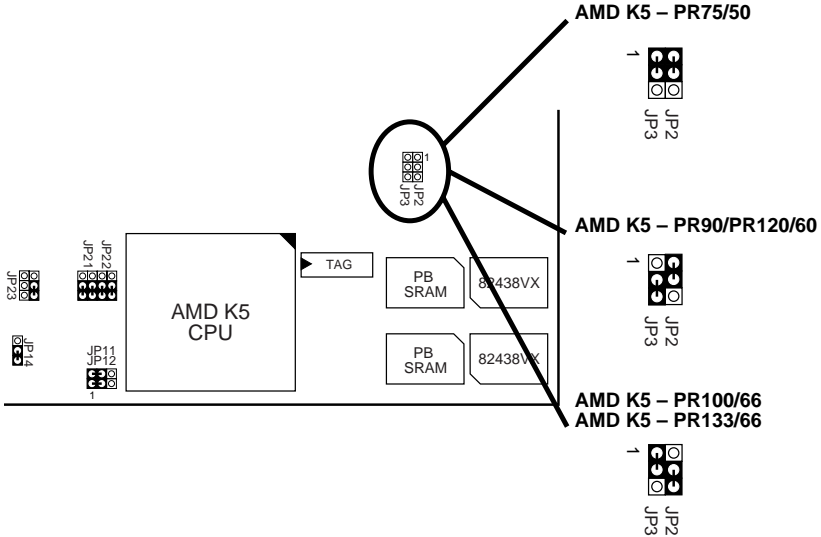
Figure 2–10. AMD K5 CPU Type Configuration
