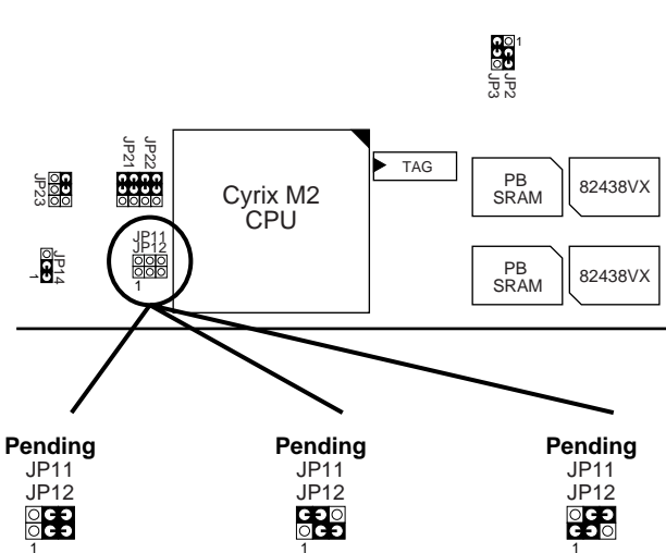
Figure 2–3. Cyrix M2 CPU Type Configuration
