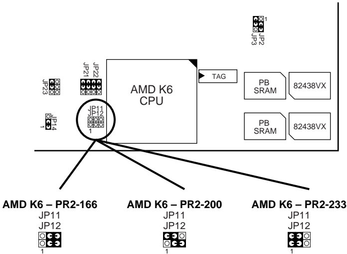
Figure 2–2. AMD K6 CPU Type Configuration
