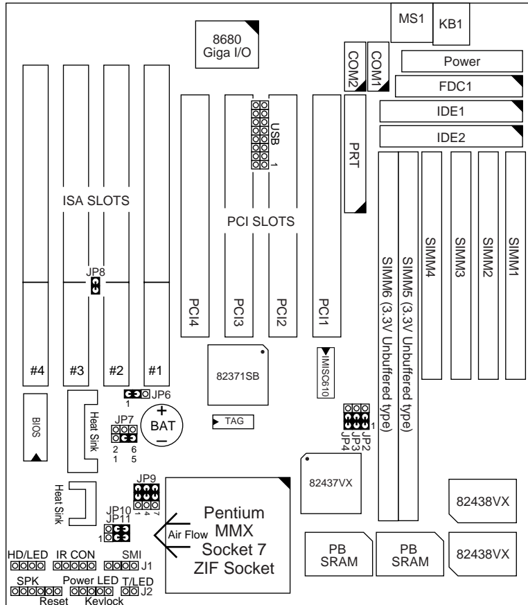
Figure 1-1. SL-54A2/A5 Motherboard Layout
