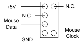
MS1 Top View
